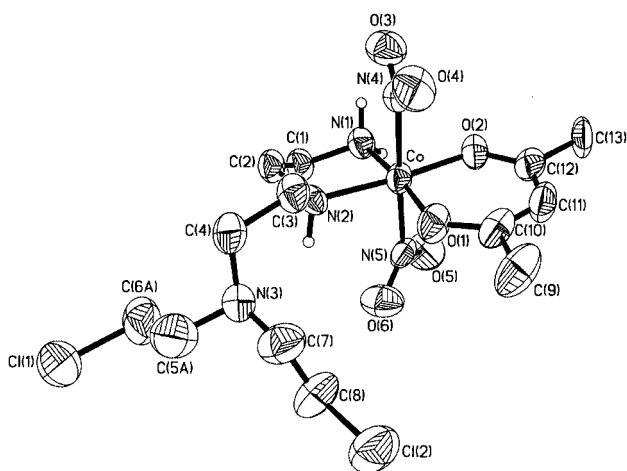
Fig. 1 ORTEP view and atomic labeling scheme of the trans - [\text{Co}(\eta^2\text{-DCD})(\text{acac})(\text{NO}_2)]^+ cation ( 9 ). Selected bond lengths (Å): Co–O(1) 1.869(7), Co–O(2) 1.887(6), Co–N(1) 1.932(8), Co–N(5) 1.946(8), Co–N(4) 1.954(8), Co–N(2) 1.965(7).
