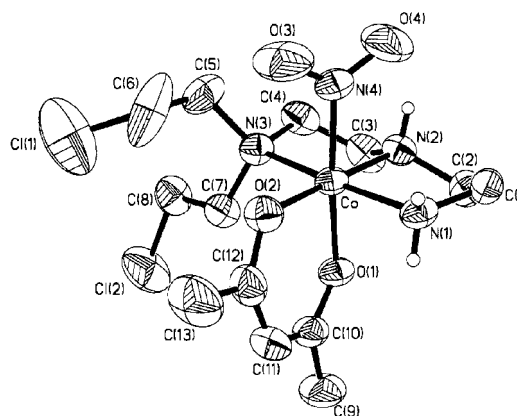
Fig. 2 ORTEP view and atomic labeling scheme of the mer - [\text{Co}(\text{DCD})(\text{acac})(\text{NO}_2)]\text{ClO}_4 cation ( 10 ). Selected bond lengths (Å): Co–O(2) 1.885(3), Co–O(1) 1.913(3), Co–N(4) 1.923(3), Co–N(2) 1.927(4), Co–N(1) 1.946(4), Co–N(3) 2.114(4).
