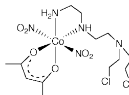
9 X = H, trans - [\text{Co}(\eta^2\text{-DCD})(\text{acac})(\text{NO}_2)]^+
