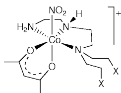
8 X = H, mer - [\text{Co}(\text{DED})(\text{acac})(\text{NO}_2)]\text{ClO}_4 10 X = Cl, mer - [\text{Co}(\text{DCD})(\text{acac})(\text{NO}_2)]\text{ClO}_4
